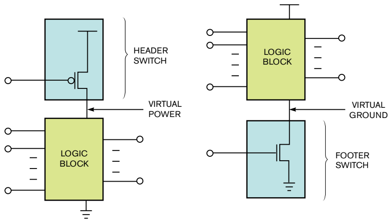
Figure 5 In MTCMOS and power gating, designers place a power-gating transistor in the stack between the logic transistors and either power or ground, thus creating a virtual supply rail (a) or a virtual ground rail (b).
