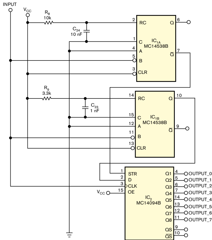
Figure 3 This circuit uses another serial-in/parallel-out register, the 4094, which has a strobe input to allow simultaneous updates of all outputs without temporary levels.
