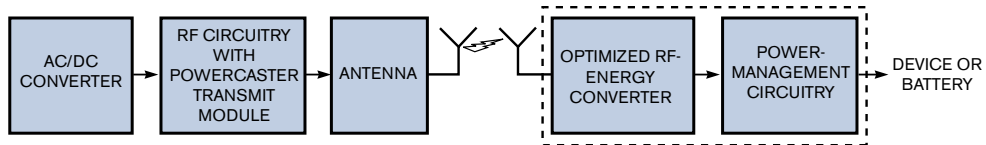
Figure 2 The Powercast RF-transmission platform comprises a Powercaster transmitter and a Powerharvester receiver. The power output is less than 100 mW, but that amount is sufficient to charge an internal battery in a wireless-sensor node or even a small, handheld consumer-electronics device.
