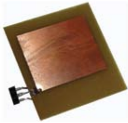
Figure B The newly developed, 28×31-mm rectenna is more compact, uses a single-layer PCB, and has an efficiency of 52%.
