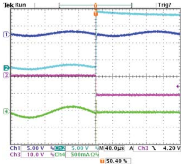
Figure 2 In Figure 1, one of IC 1 's two audio outputs (Trace 1) has protection when its external terminal accidentally contacts an 18V supply voltage (Trace 2).
