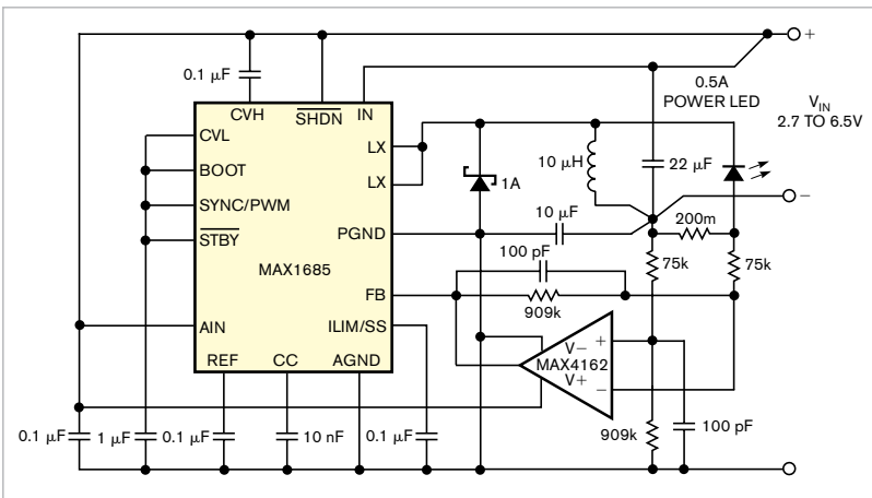
Figure 3 Another miniature, high-power LED driver delivers 0.5A and operates on 2.7 to 6.5V.
