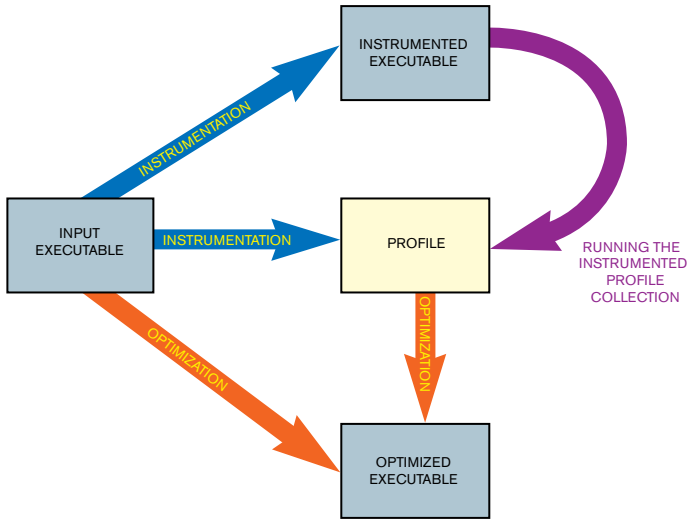
Figure 1 FDPR-Pro takes an executable program as input.
