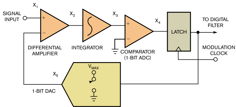
Figure 1 With a first-order modulator at the input of a delta-sigma converter, the ideal SNR is 6.02N + 1.76 - 5.17 + 30 \log_{10} \text{OSR} .
