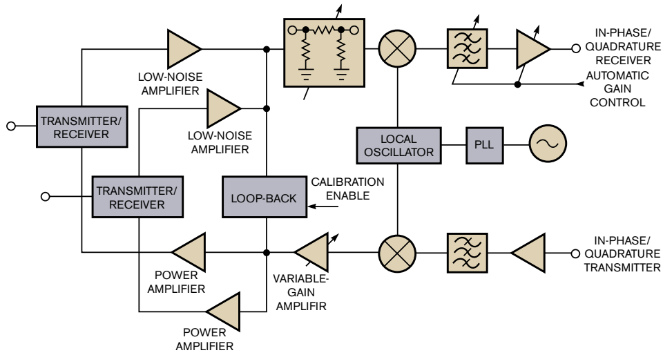
Figure 3 The 10-GHz Alereon ultrawideband-radio chip exemplifies the most common receiver architecture: the directly coupled receiver.
