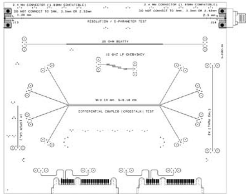
Figure 2 A typical TDR demo board (a and b) includes a resolution structure (c). The arrows highlight discontinuities created by two pairs of vertical bars—the left-hand pair separated by 1.25 mm; the right-hand pair, by 2.5 mm.
