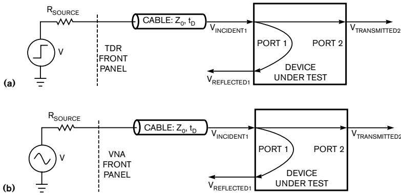
Figure A The main conceptual difference between TDR- (a) and VNA-based (b) systems is the use of a wideband, steplike source for TDR versus a narrowband sine-wave generator for VNA.
