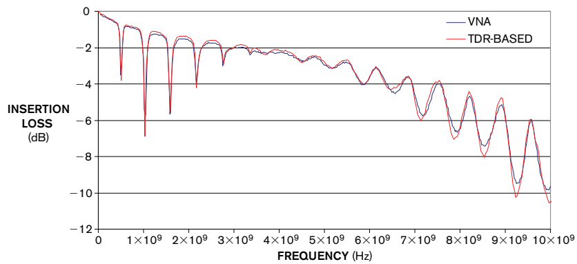
Figure B The insertion loss of VNA versus TDA shows excellent correlation (courtesy Samtec).
