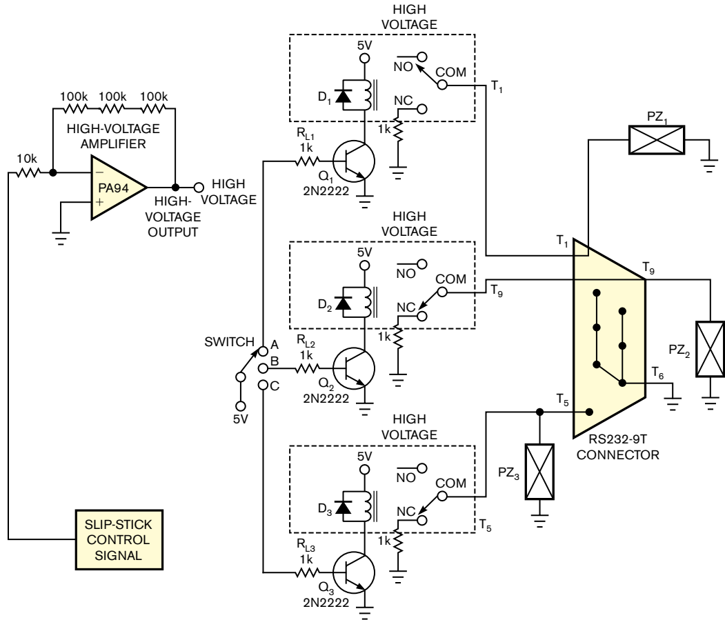
Figure 1 This simple circuit connects unenergized inputs to ground through a resistor.
