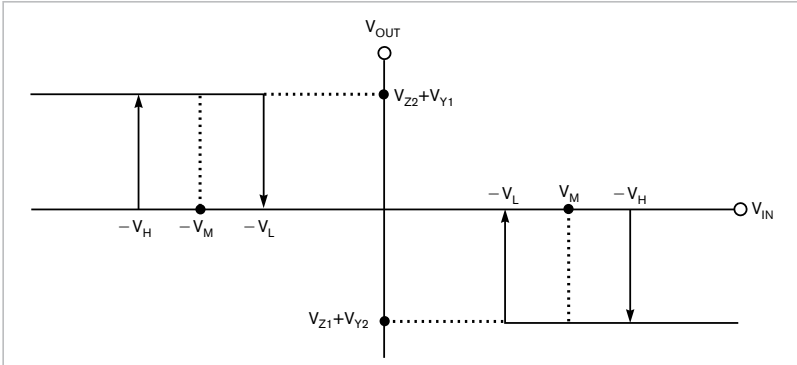
Figure 2 The I/O-transfer characteristic of the circuit in Figure1 exhibits two hysteresis bands.
