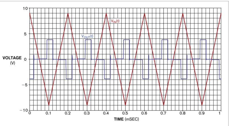
Figure 5 This oscilloscope trace shows the response of the circuit in Figure 3 to a triangular input waveform.
