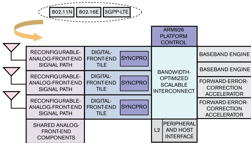
Figure 2 IMEC researchers envision an array of on-the-fly reconfigurable resources shifting instantly between air interfaces and channel conditions as bandwidth needs change.
