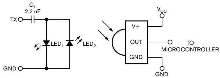
Figure 1 By sending appropriate hex values to a PC's serial port, this circuit generates precise bursts of 38.4-kHz data.
