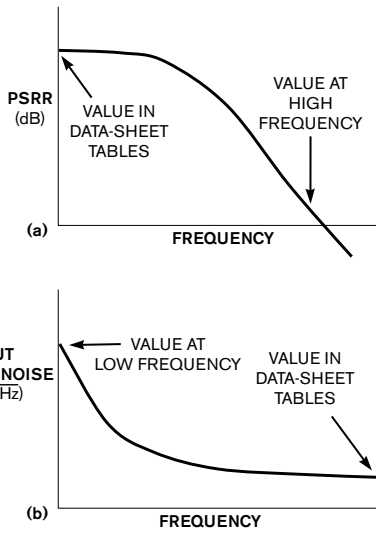
Figure 3 Data-sheet tables often overstate performance. The data-sheet tables list PSRR at dc, at which it is rarely an issue. The data-sheet chart shows where PSRR falls off drastically at high frequencies (a). Similarly, the tables list the input-voltage noise at higher frequencies where the noise is in the flat band (b).
