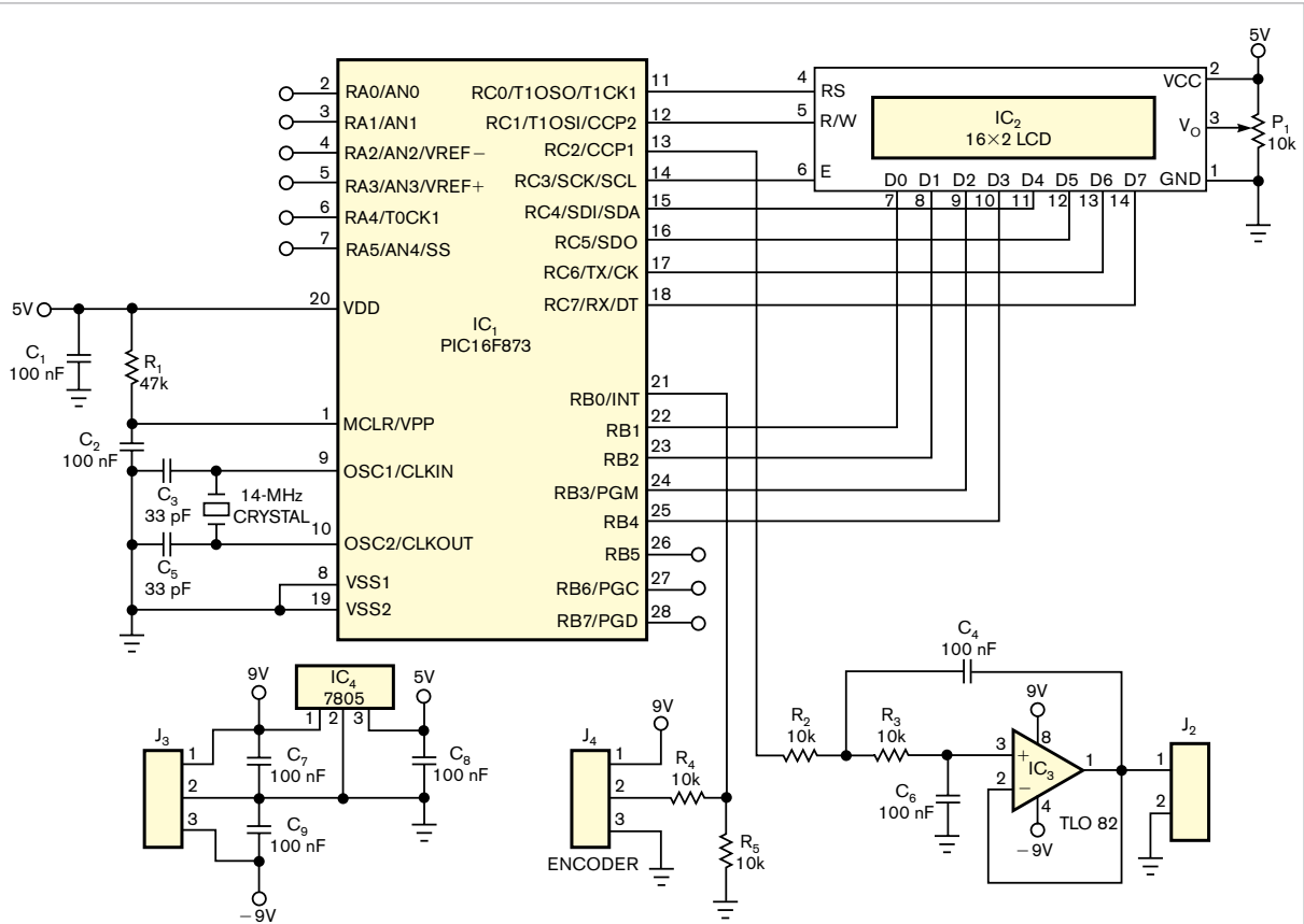
Figure 1 This circuit for measuring a motor's speed includes a PIC microcontroller and an LCD. It also provides an analog-to-digital conversion without an ADC.
