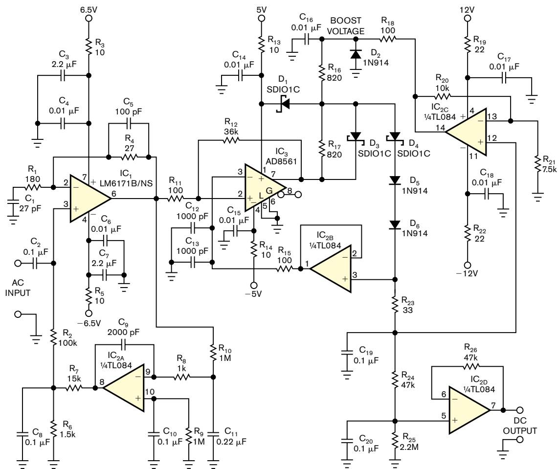
Figure 1 This precision peak detector uses an ultrafast comparator to achieve high accuracy over a wide input-frequency range.
