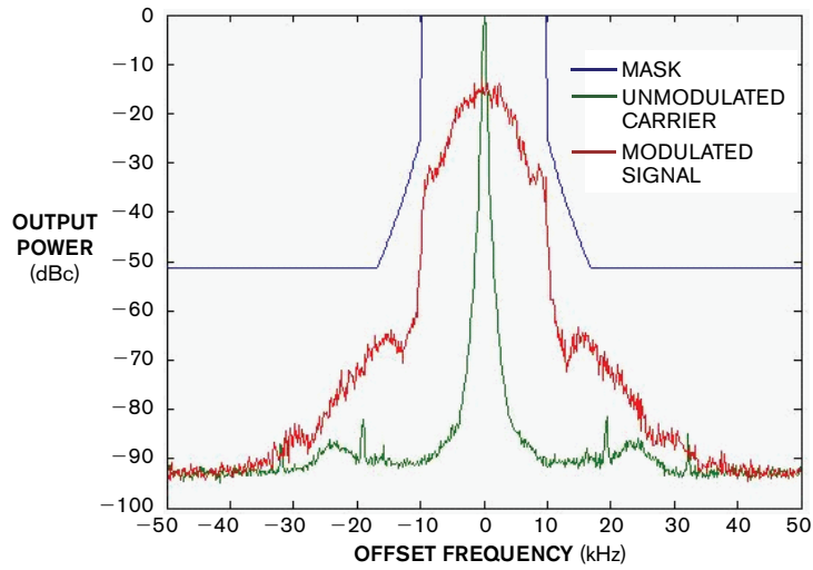
Figure 2 A sample spectral mask, 47 CFR 90.210 G, has a normalized X axis to show the offset from the center of the channel and a normalized Y axis to show the unmodulated carrier output.
