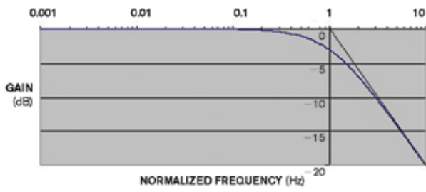
Figure 1 A single-pole function has a pole at 1 Hz.
