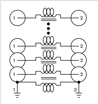
Figure 2 You can extend the passive approach in Figure 1 to multiple channels at the expense of a large magnetic component.
