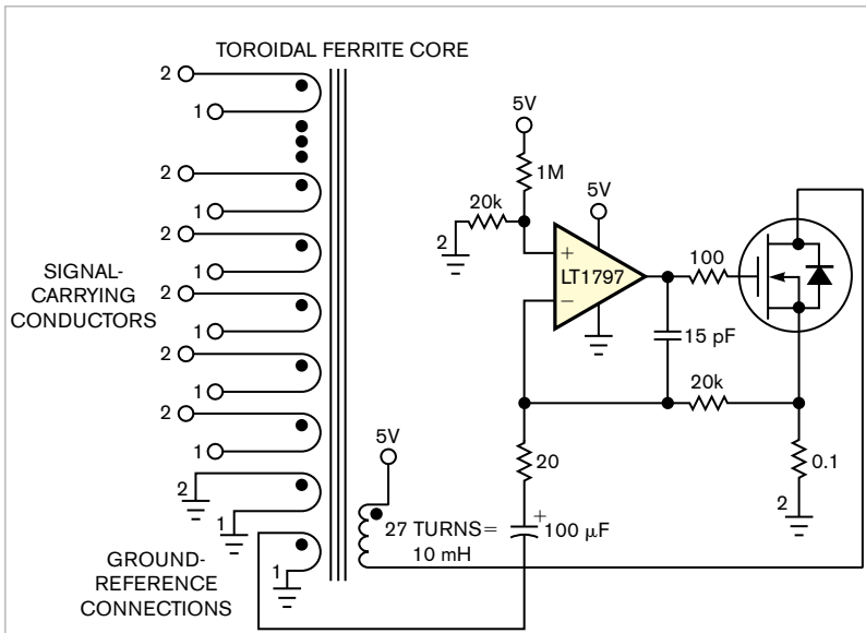
Figure 3 Using the active drive of the CMV core, you can achieve CMV reduction of 40-dB or more cancellation, extending from tens to millions of hertz.
