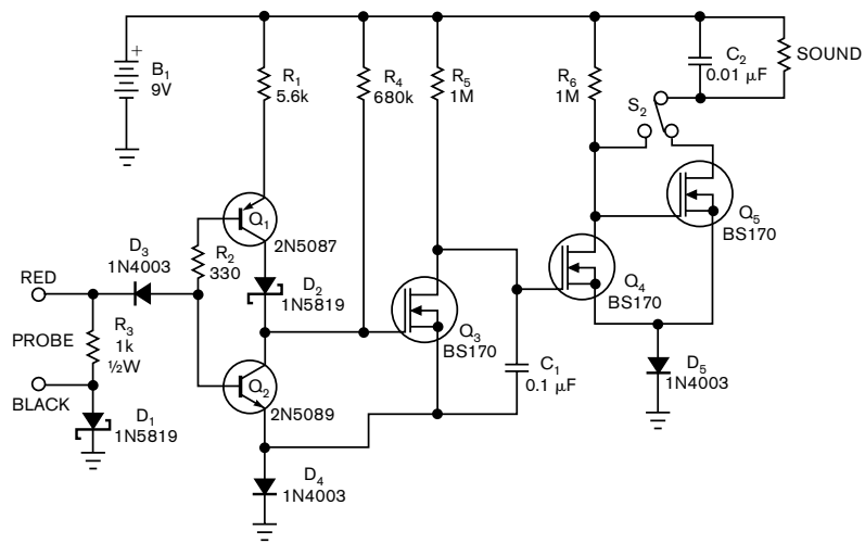
Figure 1 This simple continuity tester is switch-selectable to sound on either shorts or opens. It prevents a user from accidentally connecting it across live circuits.
