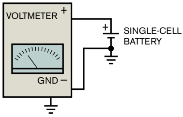
Figure 1 Common-mode voltage does not affect a voltmeter measuring a ground-referred single cell.
