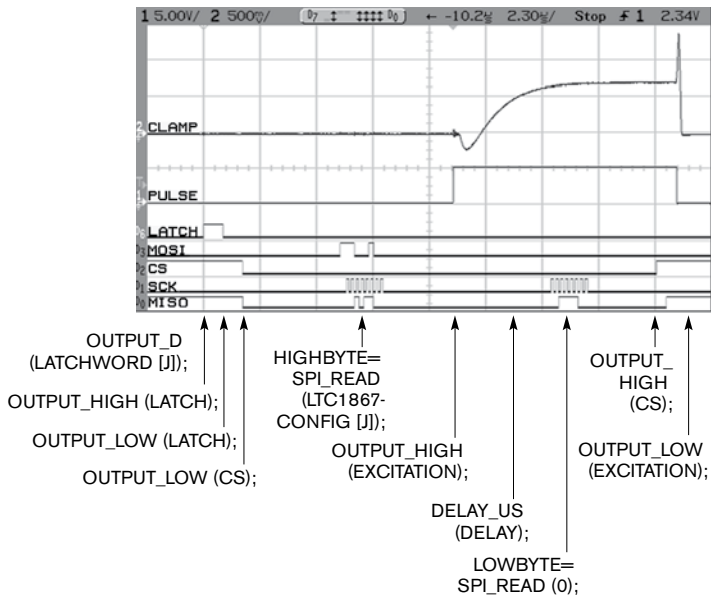
Figure 11 The interrupt-service routine monitors digital signals, excitation pulse, and clamp voltage at the ADC input along with the C code that performs these operations.
