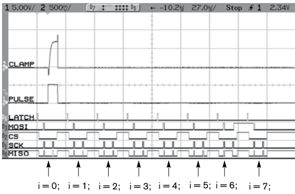
Figure 12 The interrupt-service routine scans eight channels.
