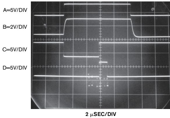
Figure 5 Figure 4's waveforms include the pulse-generator input (Trace A), the T_1 primary (Trace B), the 74HC123's Q2 delay-time output (Trace C), and S_1 's control input (Trace D). Timing ensures that sampling occurs when T_1 settles in the clamped state.
