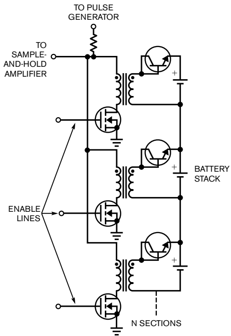
Figure 7 Adding enable lines and transistor switches facilitates multiple channels.
