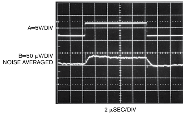
Figure C The battery-simulator output (Trace B) responds to Trace A's transformer-clamp pulse. Closed-loop control and the 680- \mu F capacitor maintain the simulator output within 30 \mu V. A noise-averaged, 50- \mu V/division sensitivity is necessary to resolve a response.
