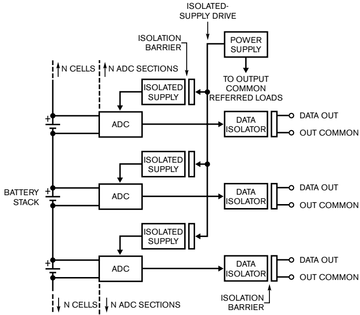
Figure D An ADC per cell requires isolated supplies and data isolators. Multiplexed-input ADCs can minimize ADC usage. You can reduce but not eliminate the isolated-supply population.
