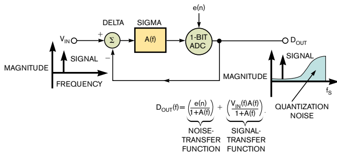
Figure 2 In a frequency-domain representation, the noise characteristic is key to the modulator's frequency operation.
