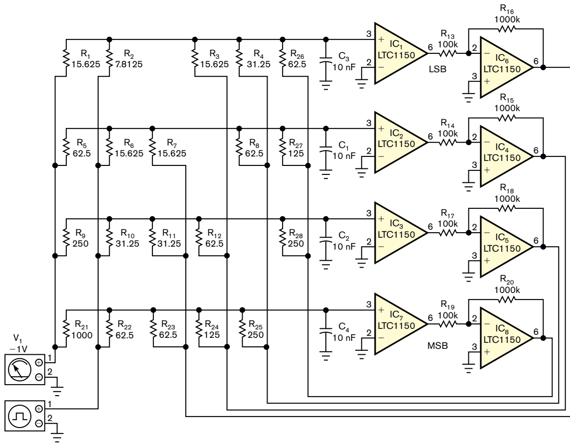
Figure 1 This Hopfield neural ADC provides a robust output in the presence of noise.
