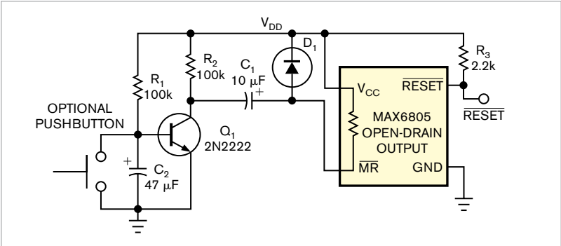
Figure 1 This simple circuit automatically resets a microcontroller upon power-up.
