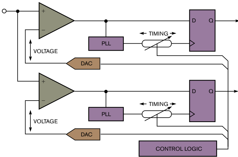
Figure 2 Vitesse has recently taken receiver instrumentation a step further, devising an interesting two-channel approach.
