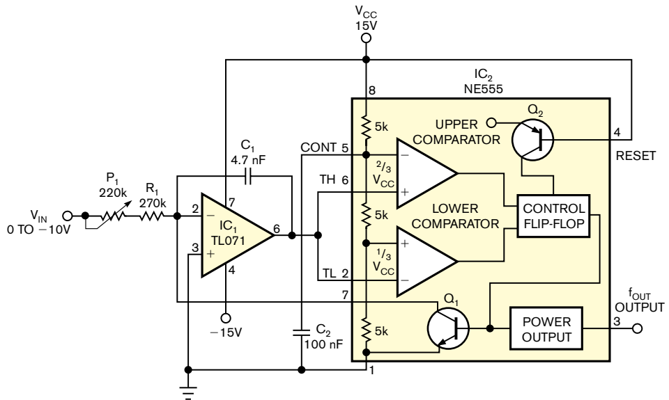
Figure 1 Preceding an NE555 timer with a Miller integrator yields a voltage-to-frequency converter that costs less than 50 cents.
