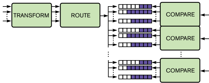
Figure 5 You can also use the VMM data scoreboard to verify multi-stream designs with user-defined data transformation and input-to-output stream routing.
