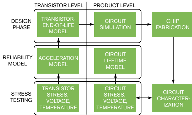
Figure A Xilinx and other large companies examine reliability at multiple phases in IC development.
