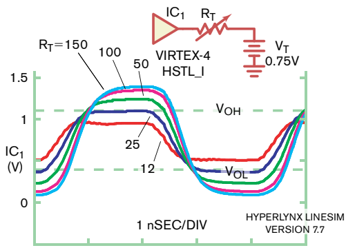
Figure 1 Reducing the value of R_T shrinks the output voltages.
