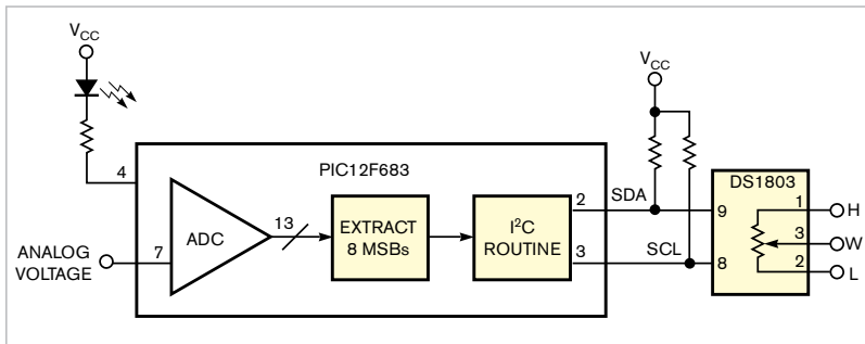
Figure 1 This circuit allows an analog-voltage input to select the digital potentiometer's resistance.
