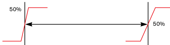
Figure 1 A trip point is the percentage of logic-high levels engineers use as a reference to measure slew (a) and delay (b) values.
