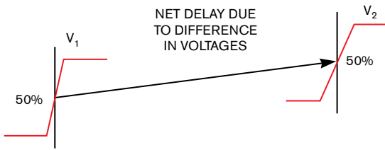
Figure 5 Without a timing model available for the ports, users must manually define a default trip point (a) and voltage level (b) to help the tool calculate the delays.
