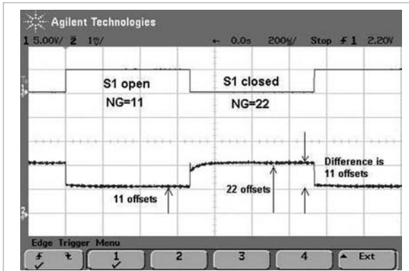
Figure 3 This oscillogram shows the output of the circuit in Figure 2, with an input voltage of 0V (grounded). The top trace is "S," the control signal applied to S_1 at 750 Hz. The bottom trace is the output error alternating between 1 and 2 mV.
