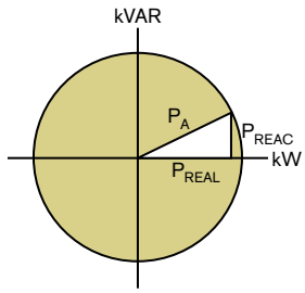
Figure 1 Power factor is the ratio of real-to-apparent power and is a measure of grid-use efficiency.
