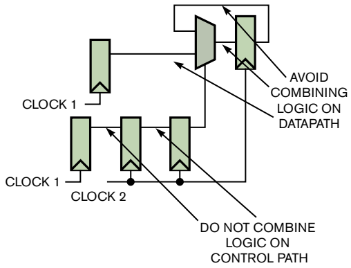
Figure 2 A good design practice is to avoid using any logic, except the recirculation-multiplexer logic, which is part of the enable flip-flop, on the datapath CDCs.
