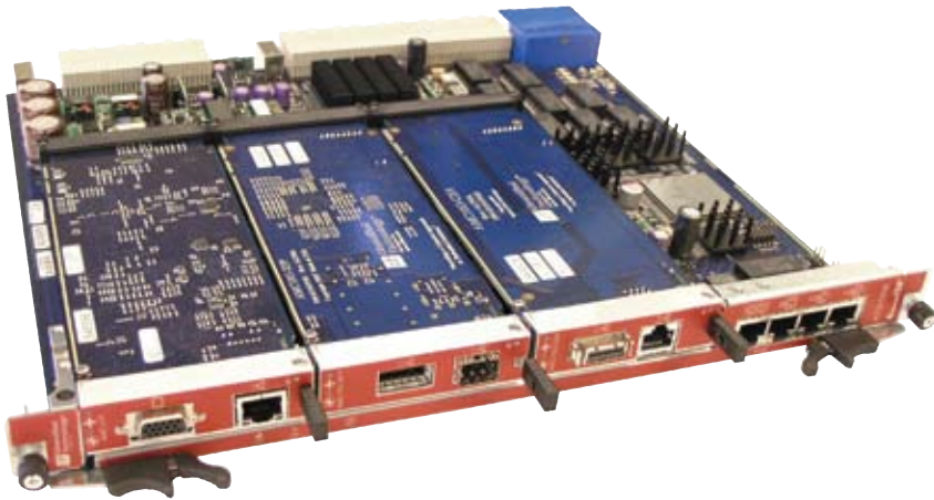
Figure 2 The ATS1936 ATCA Switch Blade features separate base and fabric gigabit-GbE networks plus three onboard AdvancedMC module sites.
