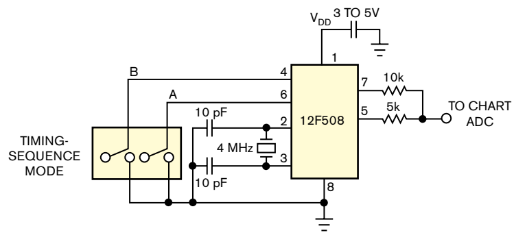
Figure 1 An 8-bit microcontroller with output pins 5 and 7 configured as a 2-bit DAC provides precise timing ticks to annotate captured data.
