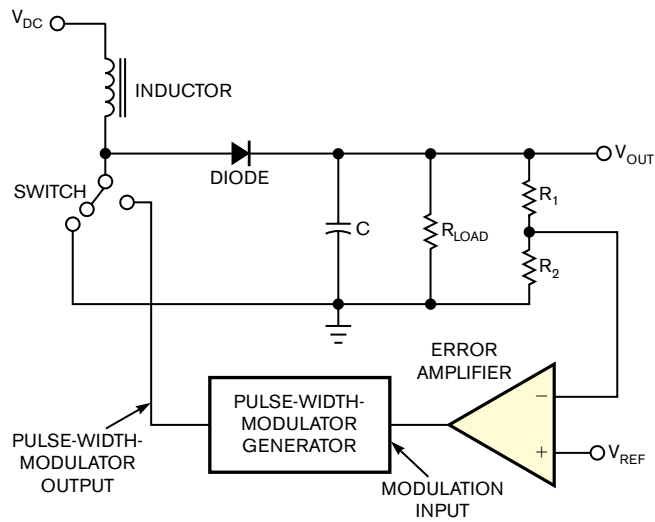
Figure 1 The output voltage in a boost switching regulator is more than the input voltage. The boost switching regulator operates in either CCM (continuous-conduction mode) or DCM (discontinuous-conduction mode)
