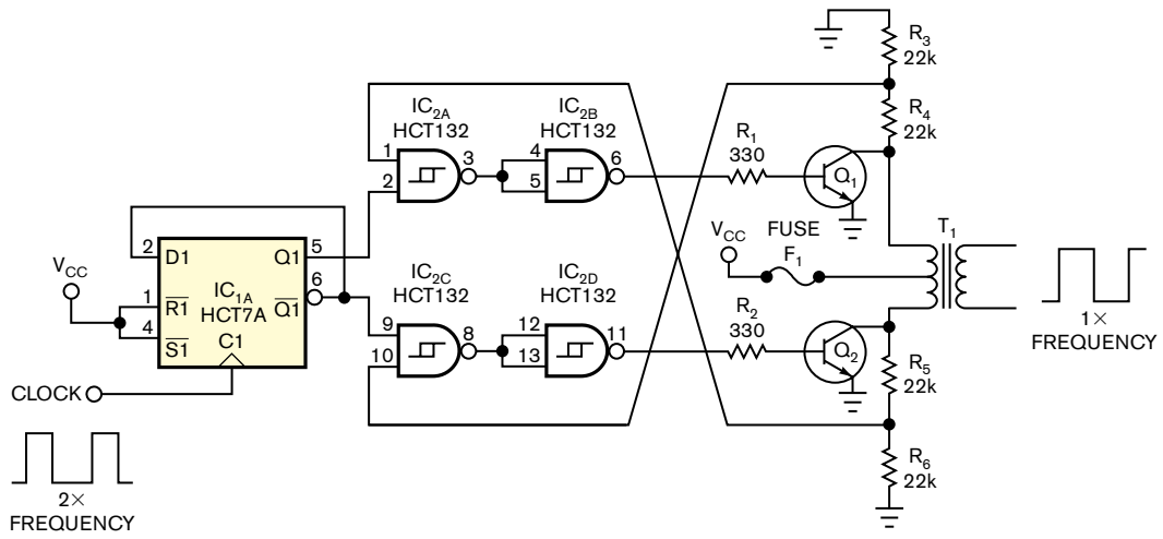
Figure 1 Cross-coupled gates prevent one transistor from turning on before the other turns off. Fuse F 1 protects against catastrophic failures.
